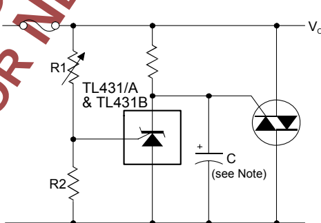
Figure 19 – Crowbar Circuit
